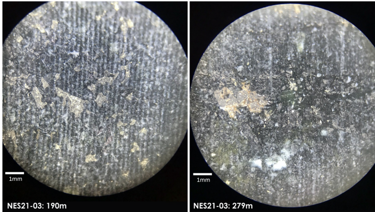
Figure 1 – Hole NES21-03 Pentlandite + Pyrrhotite in serpentinized dunite Microscope photos at 190 and 279 metres
