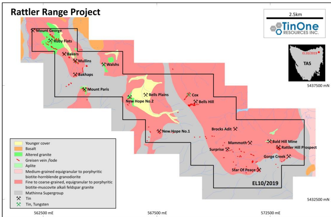
Figure 2: Rattler Range tin project summary geology and key prospects
