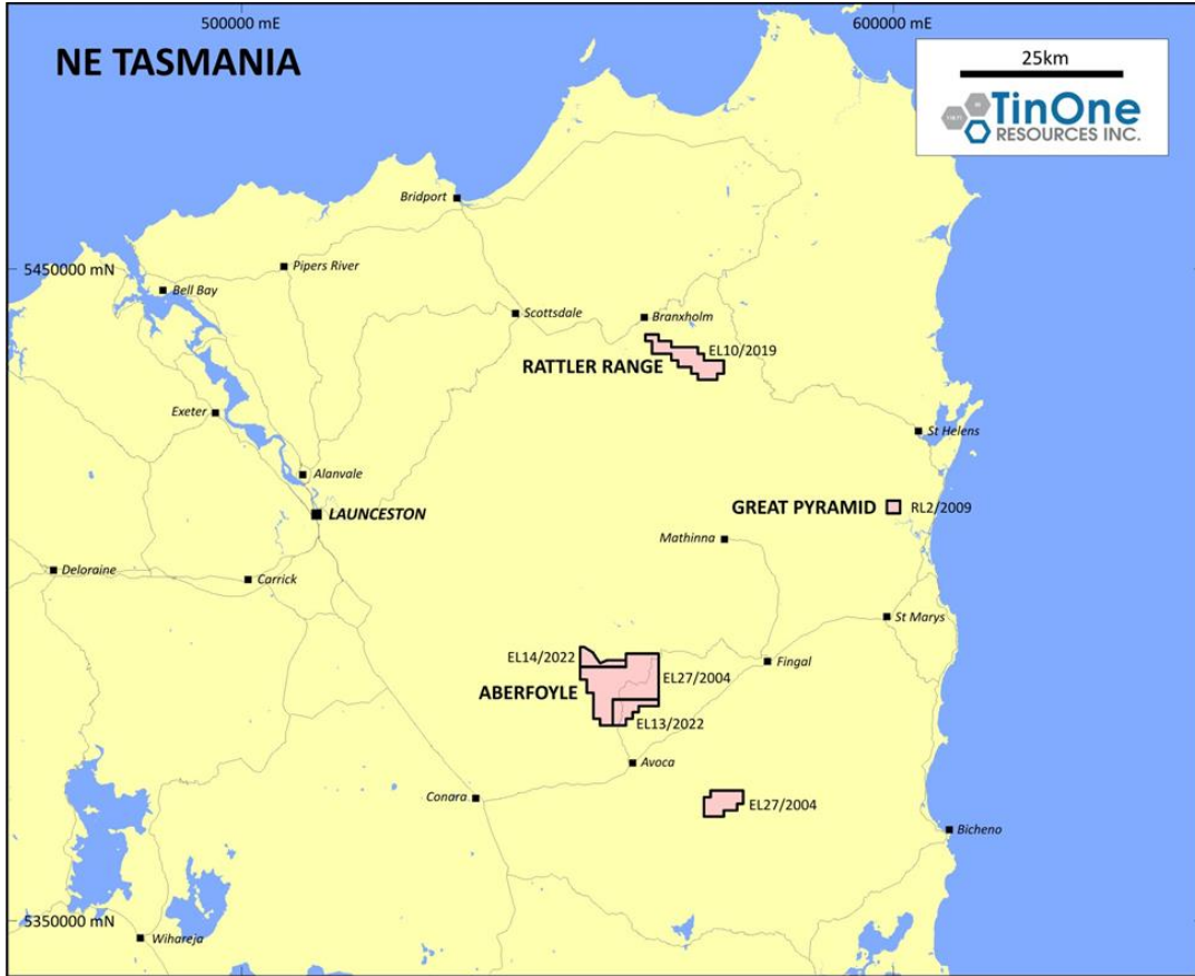
Figure 1: Rattler Range tin project location
